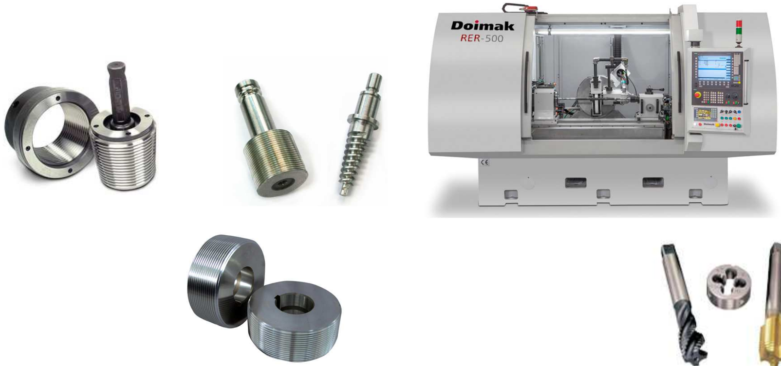
Doimak RER 500 SL Profile Grinding Machine
